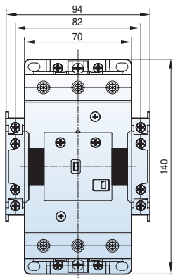
MC-75a-100a AC 2a2b + ML-150
