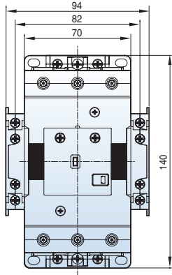
MC-75a-100a DC 2a2b + ML-150
